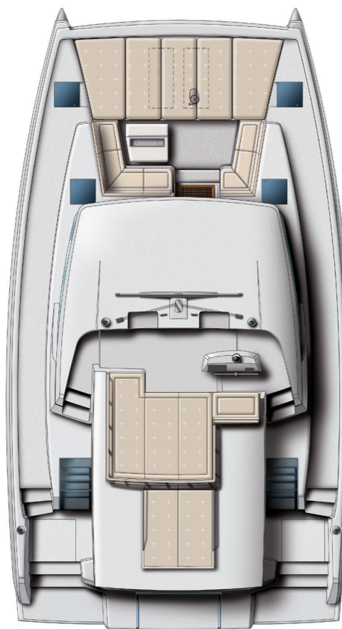
DECK AND FLYBRIDGE PONT & FLYBRIDGE
