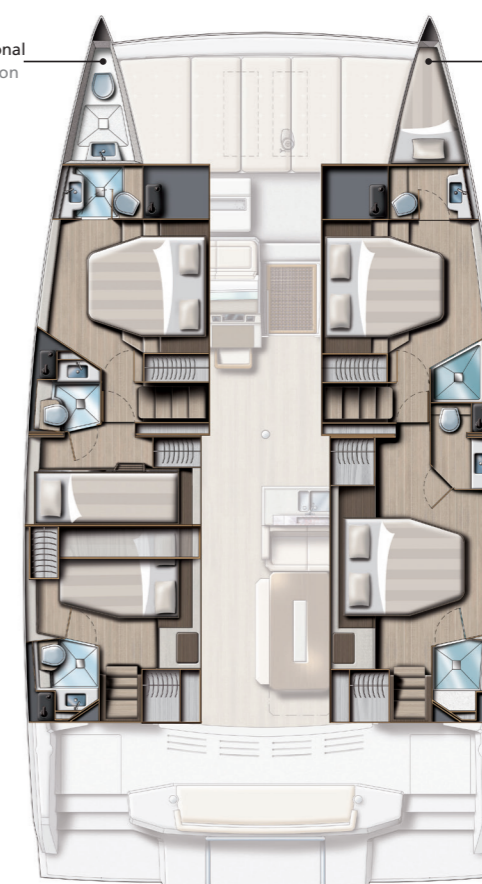
5 CABINS (4 DOUBLE + 1 TWIN) / 5 HEADS VERSION VERSION 5 CABINES (4 DOUBLES + 1 TWIN) / 5 SDB
