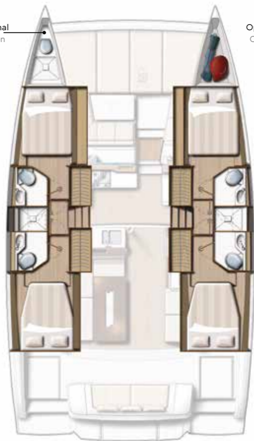
4 DOUBLE CABINS / 4 HEADS / 2 SHOWERS VERSION VERSION 3 CABINES DOUBLES / 3 SDB / 2 DOUCHES
